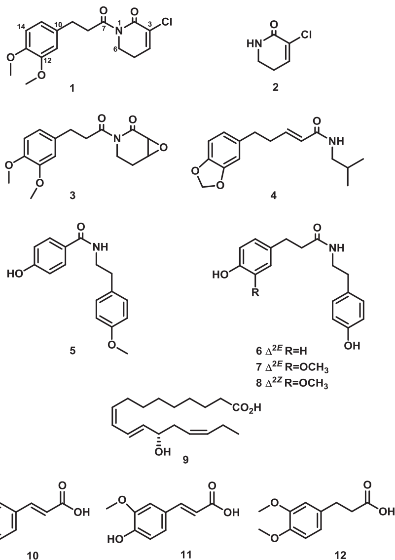
Fig. 1. Chemical structure of compounds isolated from Piper pseudoarboreum .
