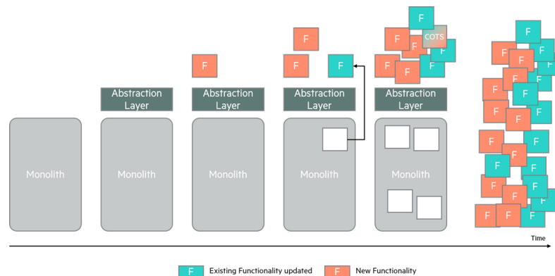
Figura 7: StranglerApplication[36]
