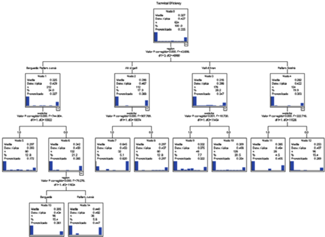
Figure 2: Decision Tree
