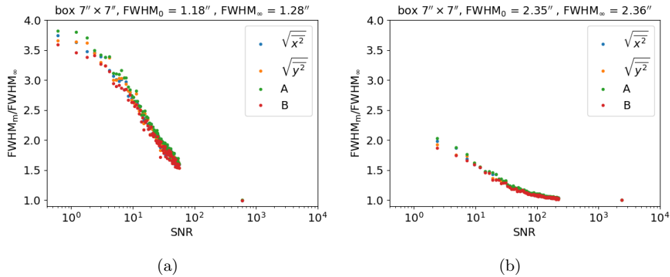
Figure 3.29: Variation of the measured size with the signal to noise ratio (S/N) of the fake object. The measured size is normalized to the value in the limit of high signal to noise. The points represent the measured size calculated using different second order moments: along the x-axis (blue), the y-axis (yellow), the major axis (green), and the minor axis of the ellipse (red). As the simulated object is symmetric, these four values should be equal, as it can be seen in the figure at high S/N. At low S/N, the noise introduces some eccentricity, making these values different. This simulation was carried out on an image of 7 \times 7 arcsec 2 with the FWHM of the simulated object set to (a) 1.18 arcsec and (b) 2.35 arcsec. It can be seen how the overestimation drops as the size of the simulated object increases.
