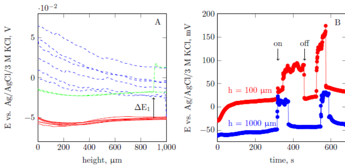
Figure 2: (A) Sequence of consecutive Z-approach curves recorded above the center of the AZ63 wire with a Mg^{2+} ISME. Step size: 10 \mu m . 500 ms settling time was allowed for the potentiometric cell at each points before measurements. Lines in chronological order: solid red = spontaneous corrosion, dashed blue = galvanic corrosion, dash dotted green = spontaneous corrosion. (B) Stationary recordings above the center of the AZ63 target with the ISME placed at: red = 100 \mu m , blue = 1000 \mu m distance from the metal. The labels On/off denote the moment when galvanic coupling was either established or ceased. Temporal resolution was 1 Hz.
