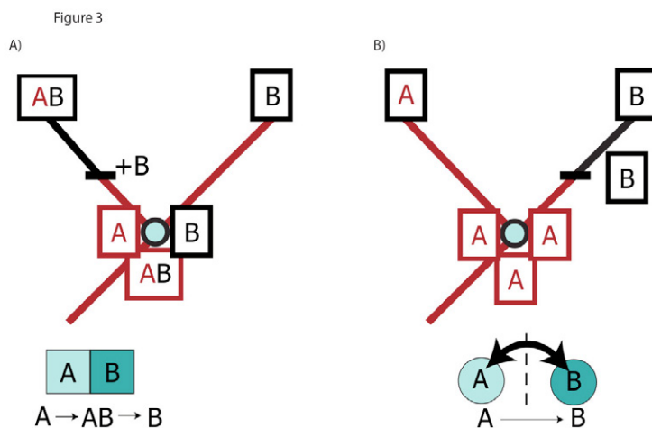
Figure 3. Two different biogeographic models underlying methods of biogeographic inference. A) Ancestral range inference models (e.g., DIVA, DEC): widespread ancestral states (AB) are allowed in the model and divided at cladogenetic events by allopatry; it is appropriate for continental scenarios in which areas are adjacent (share an edge) and gene flow is expected to be maintained; dispersal is equivalent to “range expansion”. B) Character state inference models: ancestral state inherited identically by daughters following speciation; widespread ancestral ranges not allowed and change to a new state occurs along the descendant branch; it is more appropriate for island scenarios in which dispersal is equivalent to “jump dispersal”.
