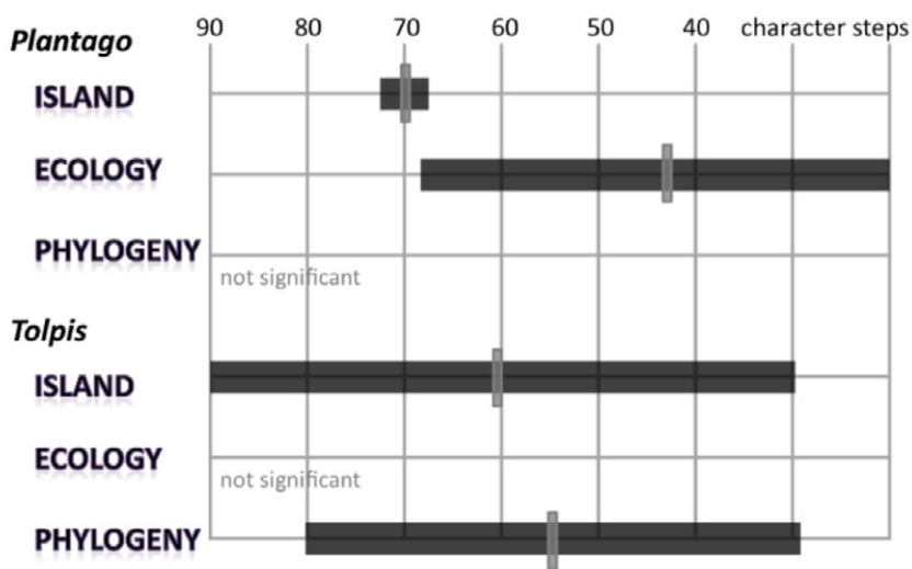
Figure 1. Summary of results of directional one-sample t-tests to evaluate significant correlations between island distribution, ecological zone or phylogeny in AM fungi and their plant hosts. The tests were performed on character reconstruction step numbers of AM fungal phylogenies; black bars represent the null distribution of randomized grey vertical bars indicate the values of the test statistic.
