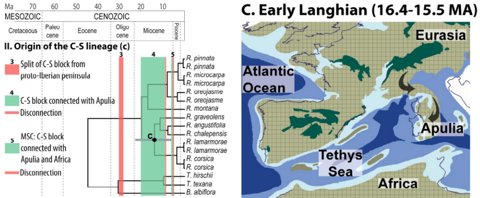
Fig 2. Origin of Corso-Sardinian endemics inferred from molecular dating and ancestral area reconstruction analyses of cpDNA sequences (modified from: Salvo G., S. Ho, G. Rosenbaum, R. Ree, E. Conti. 2010. Tracing the temporal and spatial origins of island endemics in the Mediterranean region: A case study from the citrus family ( Ruta L., Rutaceae). Systematic Biology 59: 705-722)
