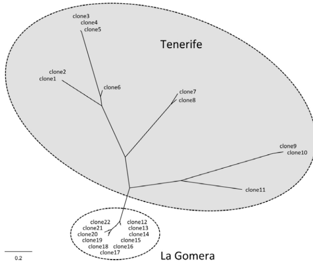
Figure 2. Maximum likelihood tree of AM fungi associated with Plantago arborescens from the laurel forest ecological zone on the islands of La Gomera and Tenerife.
