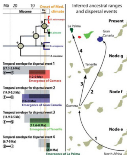
Fig 3. Origin of Canary endemics inferred from molecular dating and ancestral area reconstruction analyses of cpDNA sequences (modified from: Salvo G., S. Ho, G. Rosenbaum, R. Ree, E. Conti. 2010. Tracing the temporal and spatial origins of island endemics in the Mediterranean region: A case study from the citrus family ( Ruta L., Rutaceae). Systematic Biology 59: 705-722)
