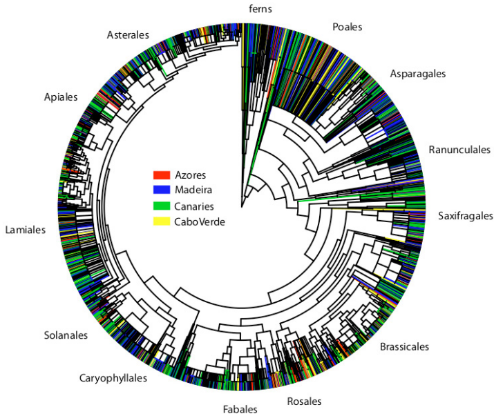
Figure 1. Time-calibrated phylogenetic tree for all 3111 vascular plant species of the Macaronesian flora based on a supermatrix-supertree approach (native species of each archipelago color-coded: Azores-red, Madeira-blue, Canary Islands-green, CaboVerde-yellow; naturalized species in black).
