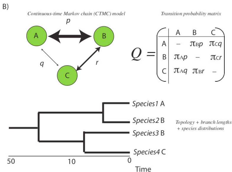
Figure 2. A) Influence of branch lengths on parametric biogeographic inference: the longer the branch length, the higher the opportunity for geographic change along the branch, and the higher the uncertainty in the inferred ancestral range. B) Parametric, model-based approach to island biogeography: range evolution is modelled as continuous-time Markov chain (CTMC) process that evolves along the branches of the phylogeny as a function of time. Transition between states is governed by an instantaneous rate matrix ( Q ), whose parameters are biogeographic processes (dispersal rates, carrying capacities). Exponentiating this rate matrix as a function of time gives the probability of geographic change from ancestor to descendants over the phylogeny ( P = e^{Qt} ).
