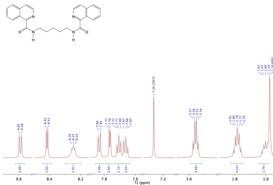
Figura 94. 1 H-RMN de Bis(1-isoquinolicarboxamido)etano (1d).
