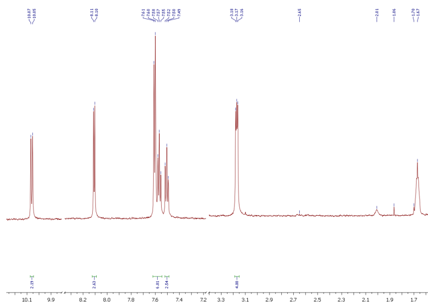
Figura 99. ^1\text{H} -RMN de [\text{Pd}(\mathbf{1b})]\cdot n\text{H}_2\text{O} ( 7b )
