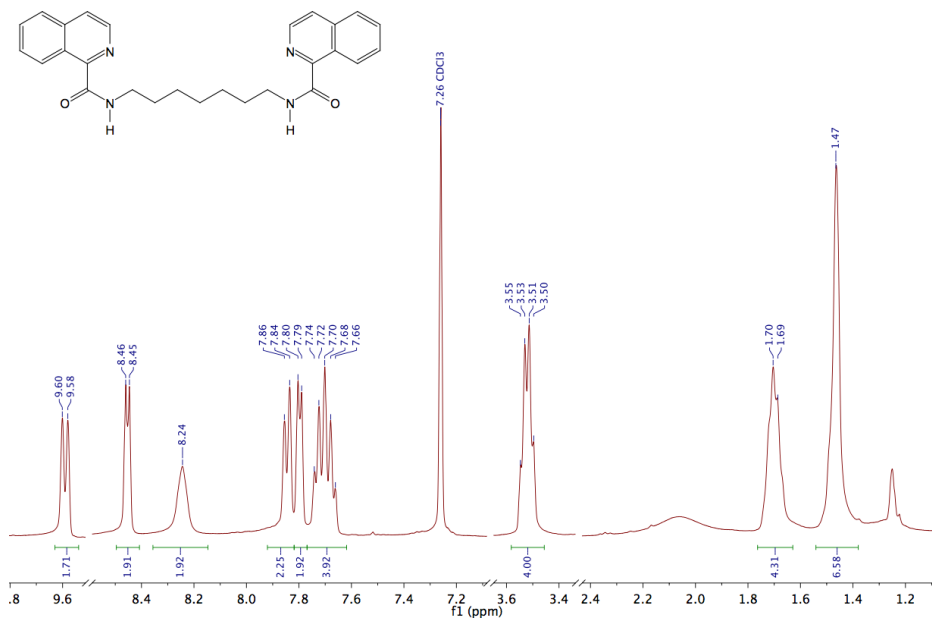
Figura 96. ^1\text{H} -RMN de Bis(1-isoquinolicarboxamido)etano ( 1f ).
