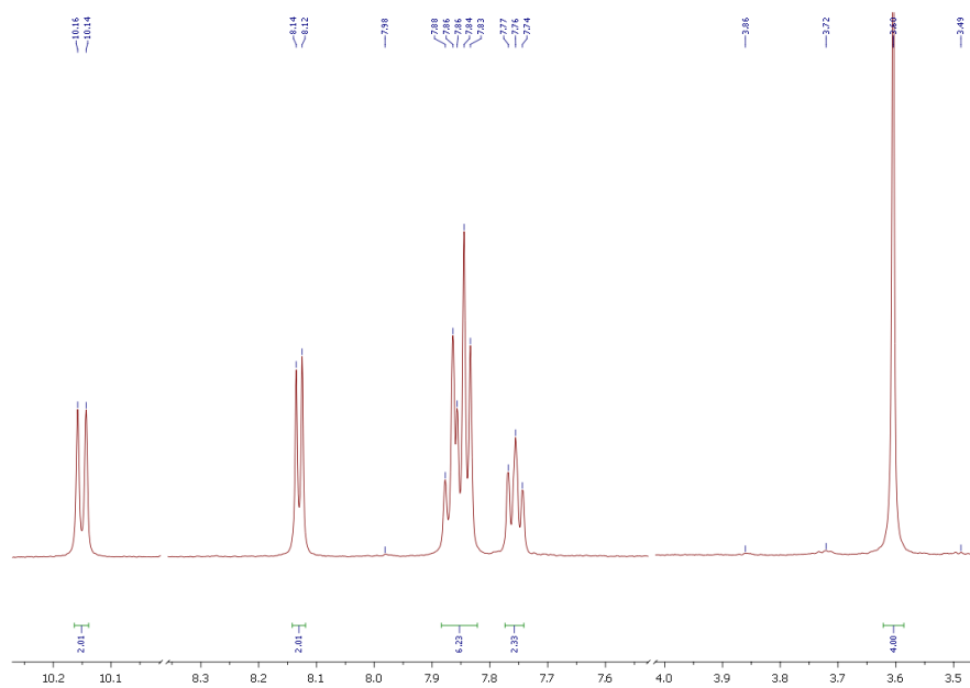
Figura 98. ^1\text{H} -RMN de [\text{Pd}(\mathbf{1a})]\cdot n\text{H}_2\text{O} ( 7a )
