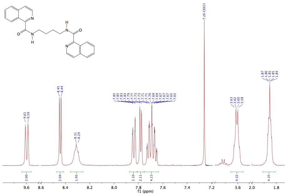
Figura 93. 1 H-RMN de Bis(1-isoquinolicarboxamido)etano (1c).
