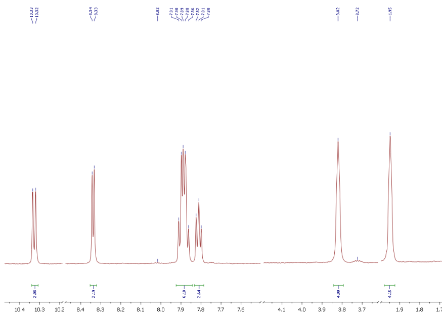
Figura 100. ^1\text{H} -RMN de [\text{Pd}(\mathbf{1c})]\cdot n\text{H}_2\text{O} ( 7c )
