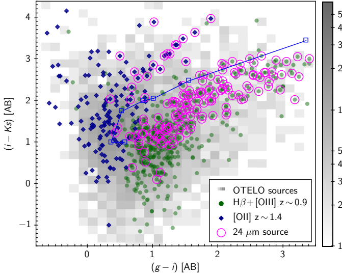
Fig. 26. (i - K_s) versus (g - i) colour-colour diagram showing the H\beta+[OIII]\lambda 4959,5007 (filled circles) and [OII]\lambda 3726,3729 (filled diamonds) emission-line candidates at z \sim 0.9 and 1.4 , respectively, selected as explained in the text. The grey background grid represents the OTELO sources and the open circles represent those sources detected with MIPS 24 \mu m . As a reference, the blue line represents a colour sequence of selected galaxy templates, described in Sect. 5.5, from E/S0 type to SB1 (open squares) at redshift z = 1.15 and E(B - V) = 0 . The reddest segment of this sequence is concurrent with the intrinsic attenuation axis.
