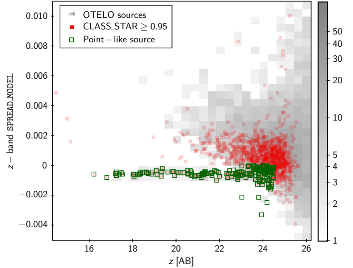
Fig. 20. Example in the z -band of the SPREAD_MODEL performance in the star-galaxy separation. Red squares represent sources with CLASS_STAR \geq 0.95 . Point sources selected (open squares) are brighter than AB = 24.5 z -band magnitude and limited by a SPREAD_MODEL value below which the star-like sequence is clear.
