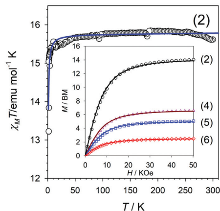
Fig. 2 Temperature dependence of the \chi_M T product for compound 2: (O), experimental; (solid line), calculated curve. The inset shows the magnetization vs. H plot at 2 K for 2, 4–6. The symbols correspond to the experimental data, whereas the solid lines correspond to the best fit to the magnetisation equation.
