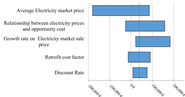
(a) Second-life battery on Wind Farm A (2027)
