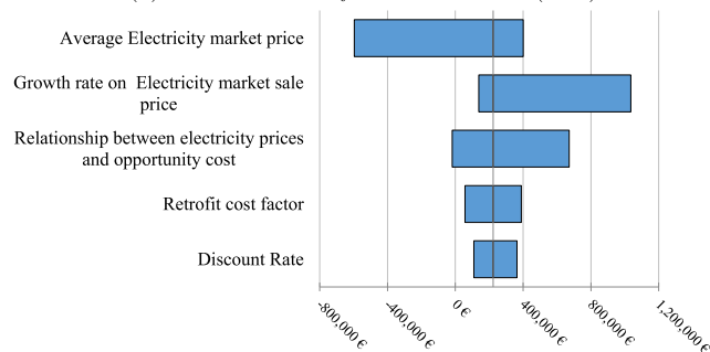
(c) Second-life battery on Wind Farm A (2031)
