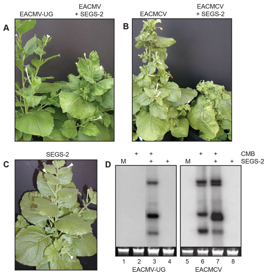
FIG 5 SEGS-2 enhances CMB infection in N. benthamiana . (A) N. benthamiana plants inoculated with EACMV-UG DNA-A plus DNA-B showed no symptoms, while plants coinoculated with EACMV-UG DNA-A plus DNA-B and SEGS-2 were symptomatic at 14 dpi. (B) Plants inoculated with EACMCV DNA-A plus DNA-B showed very mild symptoms, while those coinoculated with EACMCV DNA-A plus DNA-B and SEGS-2 displayed strong symptoms at 14 dpi. (C) Plants inoculated with SEGS-2 alone did not develop symptoms. (D) Total DNA was extracted at 14 dpi from systemically infected leaves and equivalent leaves from symptom-free plants and analyzed by DNA gel blotting with radiolabeled probes corresponding to EACMV-UG DNA-A (lanes 1 to 4) or EACMCV DNA-A (lanes 5 to 8). The lanes correspond to mock inoculation (M; lanes 1 and 5), CMB alone (lanes 2 and 5), CMB plus SEGS-2 (lanes 3 and 7), and SEGS-2 alone (lanes 4 and 8). The loading control is ethidium-stained, total genomic DNA.
