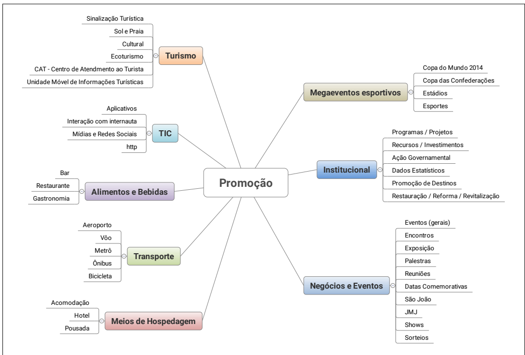
Figura 1: Code families
