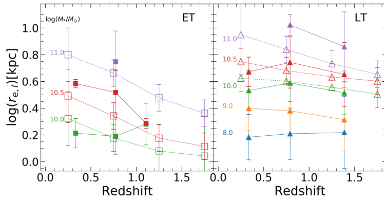
Figure 4.18. Median size evolution with redshift, the r_e - z relation. Median sizes are shown for fixed stellar-mass bins centered at \log M_*/M_\odot = 8, 9, 10.5, and 11, with colours indicated in the right side of the plots (bin width of 0.5 dex.). Note that only three most massive bins are showed for ET for each volume (left panel). Filled symbols represent data from this work, while open markers shows data from Mowla et al. (2019), given in their Table 3 (including errors). Our error bars represent the median absolute deviation of the data in each bin. We only plot the median sizes for bins which have more than 3 sources.
