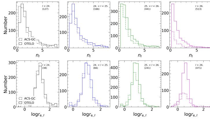
Figure 4.10. Comparison of the results from this work with those obtained by Griffith et al. (2012). Top row contains a comparison of the Sérsic index n_I distributions, while bottom row represents the logarithm of effective radius r_{e,I} . Each panel show a comparison for each magnitude bin indicated in the top-right corner. Numbers between brackets show the number of sources recovered in this work.
