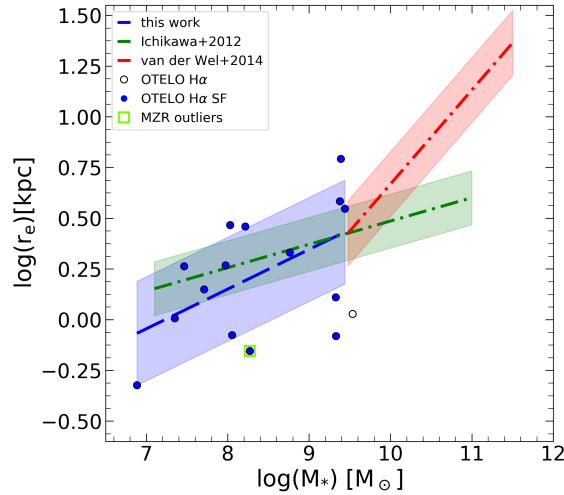
Figure 6.7. Physical half-light radius r_e as a function of the stellar mass M_* . Black empty circles show the H\alpha sample, and blue markers show SF galaxies (in both cases we show sources for which it was possible to measure both variables). The green square shows the outlier of the MZR. The blue dashed line represents the linear fit in a form y = a + bx to the H\alpha sample with a = -1.41 \pm 0.73 and b = 0.19 \pm 0.09 . The green dot-dashed line shows the linear fit from Ichikawa et al. (2012), with a logarithmic slope of 0.115. The red dot-dashed line shows the linear fit found by van der Wel et al. (2014), with a slope of 0.25. The green and red shaded regions represent the dispersion of the linear fit as estimated by Ichikawa et al. (2012) and van der Wel et al. (2014), respectively, while the blue shaded region shows the dispersion of our measurement estimated as the median absolute deviation of 0.2. Note that the sizes and stellar masses of the H\alpha sample are slightly different than those shown in Figure 4.14 due to small changes in the estimation process. We keep this figure as it is published in Nadolny et al. (2020). The overall results remain unchanged.
