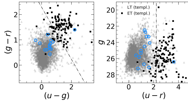
Figure 4.17. ET/LT-colour separation from Strateva et al. (2001) using data from this work. Gray triangles and black squares represents LT and ET galaxies classified via best-fitting galaxy templates. Dot-dashed line represent (u - r) = 2.22 . Blue circles represent the H\alpha sample studied in Chapter 6.
