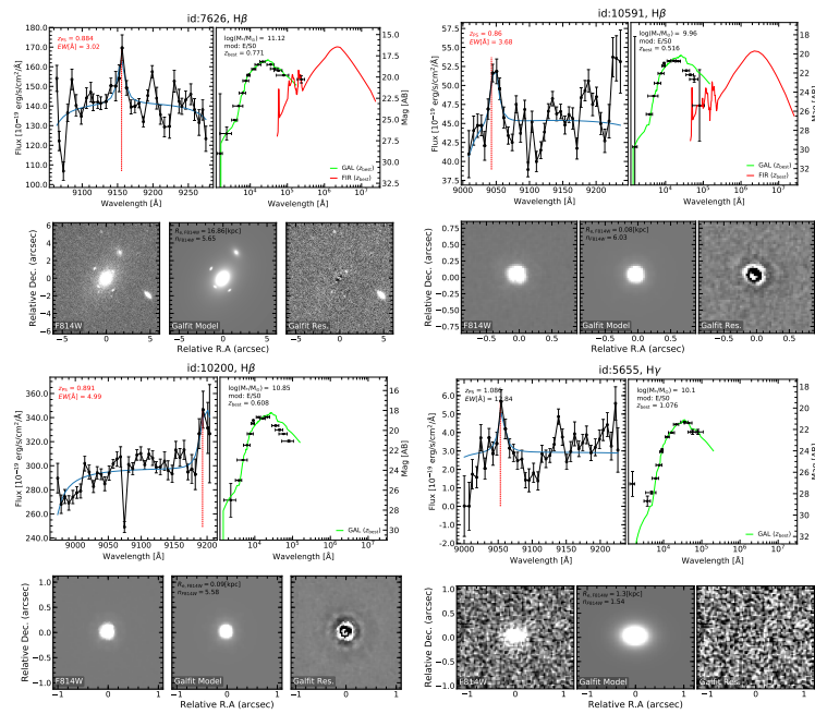
Figure 5.9. As Fig. 5.7 for Hβ and Hγ sources.
