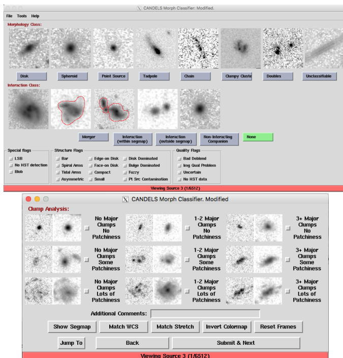
Figure 3.2. MorphGUI graphic user interface. Top panel: main morphology class, and interaction class are showed. Examples of each morphologies and interactions are displayed; specific flags showed in the lower part of this panel are available to be eventually selected. Bottom panel: Clump analysis. This window enable to select the clumpiness of the sources, as well as to navigate through the GUI (e.g., save the classification task, change to another object, etc.).
