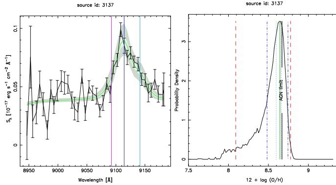
Figure 6.3. Pseudo-spectrum and metallicity PDF of source id:3137
