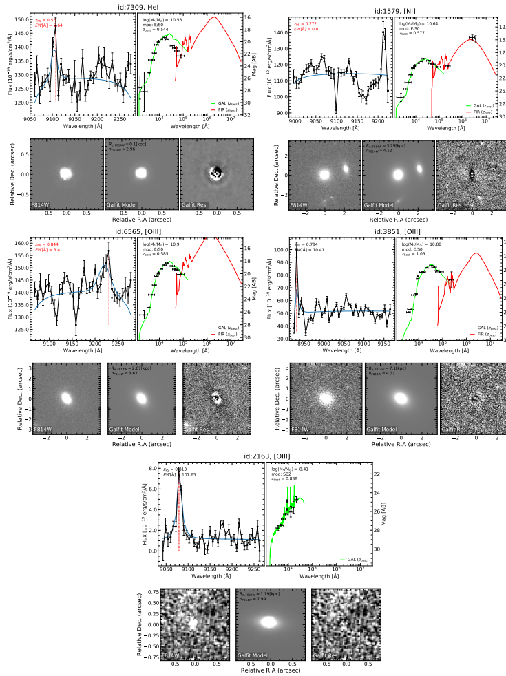
Figure 5.8. As Fig. 5.7 for He I, [N I] and [O III] sources.
