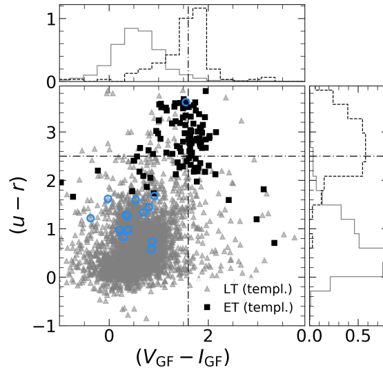
Figure 4.11. Comparison between (V_{GF} - I_{GF}) and (u - r) colours. Triangles and solid lines in gray represent LT, squares and dashed lines in black correspond to ET galaxies. Top and right-hand density histograms correspond to (V_{GF} - I_{GF}) and (u - r) , respectively. Dot-dashed lines show the results of linear discriminant analysis of both colours with (V_{GF} - I_{GF}) = 1.7 and (u - r) = 2.5 . Blue circles represent the H \alpha sample studied in Chapter 6.
