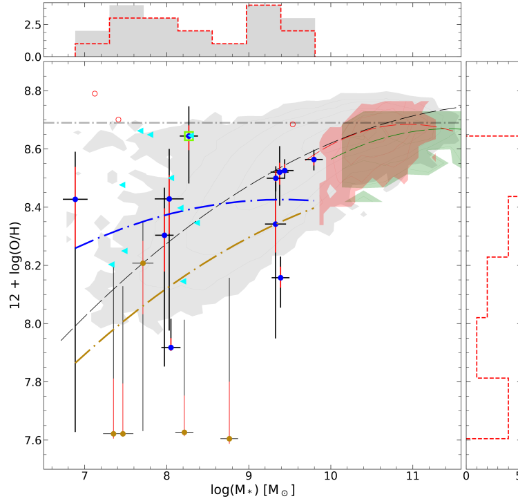
Figure 6.4. Mass-metallicity relation for OTELO H \alpha ELS. Blue and golden markers represent sources with an [N II] \lambda 6583 line flux above and below OTELO flux limit, respectively. The light green empty square shows the MZR outlier as defined by Peeples et al. (2008). Cyan triangles show the VVDS-Ultra-Deep selected sample with z_{\text{mean}} = 0.26 . Grey filled contours show local SDSS SFGs. Green filled contours show the high- z SDSS sample. Red filled contours show the SFG sample from the GAMA survey. All fits shown in this figure represent second-order polynomial fits. The blue dot-dashed line is the OTELO MZR fit to the sources with an [N II] line flux above the OTELO line flux limit, and the golden dot-dashed line shows the OTELO MZR including low-flux sources; the black thin dashed line shows the fit to the local SDSS sample; and green and red dashed lines show the SDSS and GAMA samples at z \sim 0.3 , respectively. The error bars correspond to the 25% (red) and 68% (black) confidence interval around the most probable value. The calibration uncertainty in metallicity is not included.
