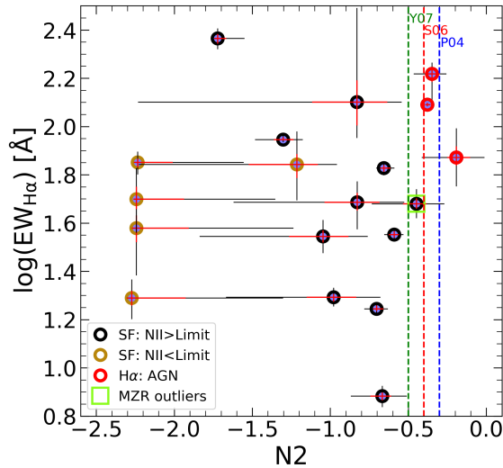
Figure 6.2. N2 index vs. EW_{H\alpha} . Blue pints show all the H\alpha candidates. Black and golden circles represent sources with an [N II] line flux above and below OTELO flux limit, respectively (see Section 6.3 and Bongiovanni et al. 2020). Red circles show AGN candidates selected using the Stasińska et al. (2006) empirical limit of N2 = -0.4 . Vertical green and blue dashed lines show the Yin et al. (2007) and Pettini & Pagel (2004) limits of their calibration using the N2 index, respectively. The red line shows the AGN selection limit from Stasińska et al. (2006). The error bars in each object correspond to the 25% and 68% confidence interval around the most probable value.
