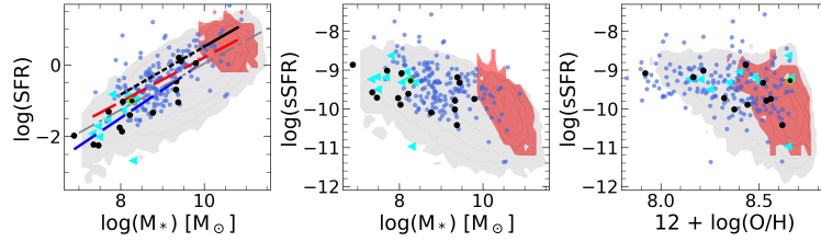
Figure 6.6. Star formation rate and sSFR as a function of stellar mass and metallicity. In all panels, black markers show the OTELO SFG sample, green empty circles show transitional dwarf galaxies, cyan triangles show the VVDS-Ultra-Deep data, blue dots show the VVDS-Deep data, and contours in red and grey show the GAMA and local SDSS samples, respectively. In the left panel we show the linear fits to our SFG sample (blue dashed line), VVDS Deep+Ultra-Deep (both selected sub-samples from VVDS, red dashed-line), and the fit from (Noeske et al. 2007, black solid line), which is given in the mass range of 10^{10} to 10^{11} M_{\odot} , and the black dashed line is an extrapolation of their fit down to 10^8 M_{\odot} . The grey dashed line shows the linear fit of the local SDSS sample. For clarity we do not plot the estimated dispersions for any fit.
