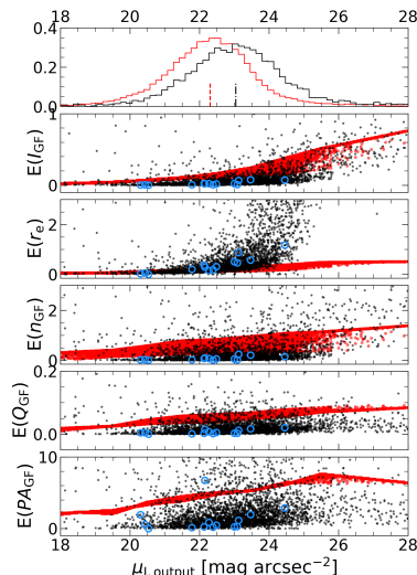
Figure 4.15. Errors of given parameter as a function of surface brightness \mu_{\text{output}} . Black dots show the outcome from this work, and the red dots show data for selected ( f=1 ) galaxies from Häussler et al. (2007). Top panels show density distribution of \mu_{\text{output}} . The median values are marked with a red dashed-line (22.3) and a black dot-dashed line (23.04). Circles in blue show the H \alpha sample studied in Chapter 6.
