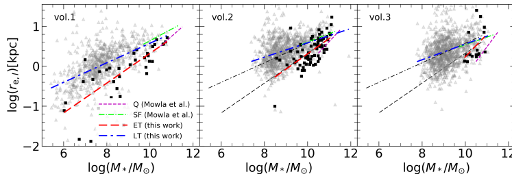
Figure 4.13. Effective radius as a function of stellar mass – the mass-size relation. Each panel correspond to selected cosmic volumes: vol1: z < 0.5 , vol2: 0.5 \leq z < 1 , and vol3: 1 \leq z < 2 . Gray triangles and black squares show LT and ET galaxies, respectively. Dot-dashed blue and dashed red lines show power-law fits for LT and ET data, respectively, according to Eq. 4.1. The best-fit parameters are given in Table 4.1. Gray dot-dashed, and dashed lines in the middle and right panels show the fits for LT and ET obtained for the first cosmic volume (vol1). Dot-dashed green and dashed magenta lines represent the LT (SF) and the ET (Q) MSR, respectively, as reported by Mowla et al. (2019).
