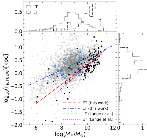
Figure 4.14. Effective radius as a function of stellar mass – the mass-size relation. Gray triangles and black squares show LT and ET galaxies, respectively. Dot-dashed blue and dashed red lines show the power-law fits for LT and ET data, respectively, according to Eq. 4.1. Thin dot-dashed green and dashed magenta lines represent the LT and ET MSR from Lange et al. (2015). Top and right panels show density histograms of stellar mass and size, respectively. Parameters of fitted power-law are given in the bottom of Table 4.1. Circles in blue shows the H \alpha sample studied in Chapter 6.
