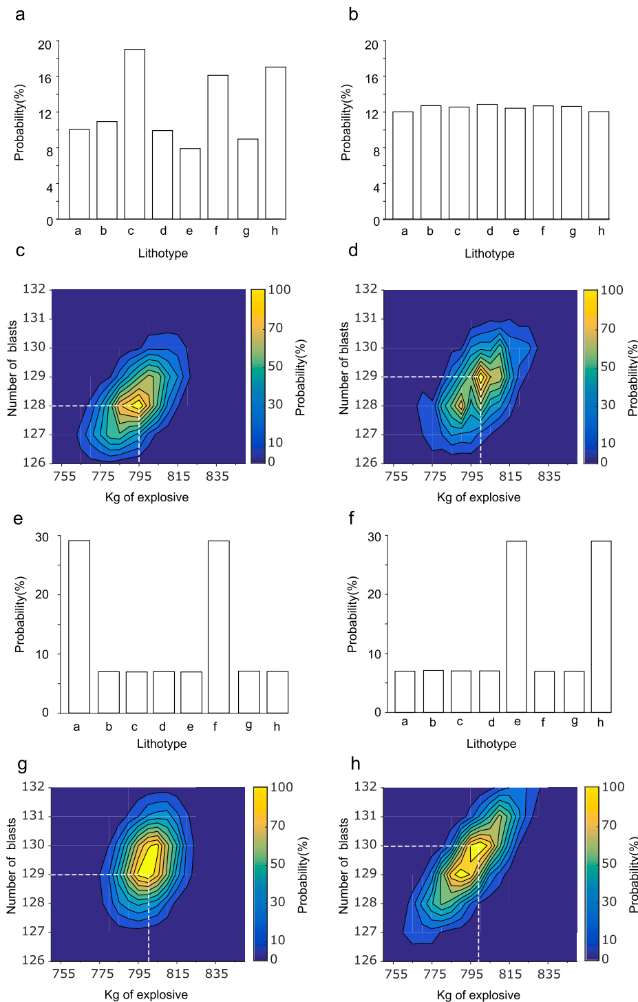
Fig. 7. Relationship between lithotype, number of blasts and amount charge of explosive calculated with the proposed mathematical model. (a), (b), (e) and (f) are the histograms with the lithotypes used in the simulated tunnels. (a) Has a distribution similar to the lithotypes found in the Güimar tunnel, (b) corresponds to a uniform distribution, (e) and (f) are proposed non-uniform distributions. (c), (d), (g) and (h) give the probability of the number of blasts and the kilograms of explosive needed for the simulated tunnels of 120 m, corresponding to the (a), (b), (e) and (f), respectively. The lithotypes are: (a) aphanitic massive basalt, (b) altered and highly altered aphanitic massive basalt, (c) vacuolar aphanitic basalt, vacuole < 0.05 mm, (d) vacuolar aphanitic basalt, vacuole < 0.3 mm, (e), phonolite, (f) red colour ignimbrite, (g) highly altered red colour ignimbrite and (h) agglomerate basaltic materials.
