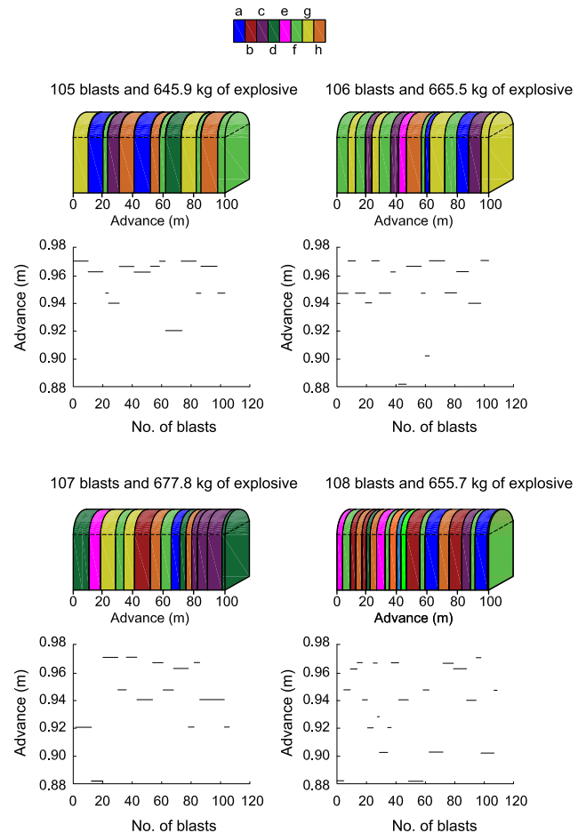
Fig. 6. Application of the mathematical model in computer simulated tunnels. The mathematical model is applied to predict the number of blasts and the amount of charge needed in four tunnels to drill 100 m. The lithotypes are: (a) aphanitic massive basalt, (b) altered and highly altered aphanitic massive basalt, (c) vacuolar aphanitic basalt, vacuole < 0.05 mm, (d) vacuolar aphanitic basalt, vacuole < 0.3 mm, (e), phonolite, (f) red colour ignimbrite, (g) highly altered red colour ignimbrite and (h) agglomerate basaltic materials.
