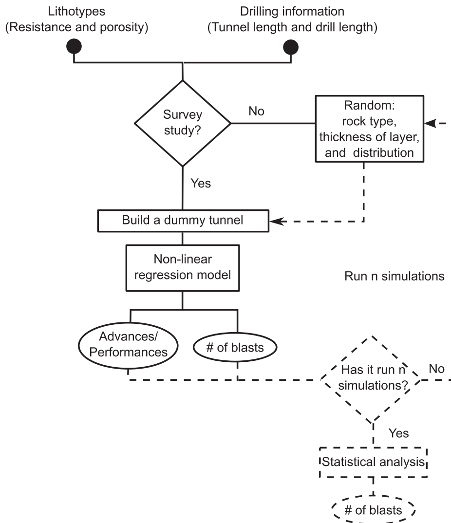
Fig. 3. Block diagram of the method. The proposed methodology is shown to estimate the powder factor according to the different lithologies of the volcanic lands.
