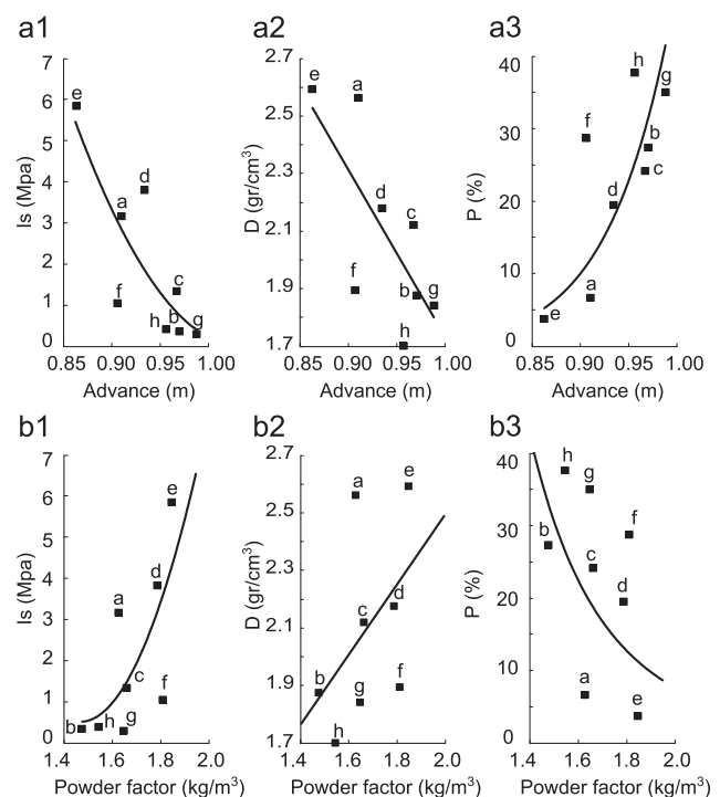
Fig. 4. Relationship between lithotype and blasting process. (a) and (b) show the relation between advance (m) and powder factor (kg/m 3 ) versus point load strength index Is (MPa), hydrostatic balance density D (g/cm 3 ) and open porosity P (%), respectively. Black lines are the fit. The lithotypes are: (a) aphanitic massive basalt, (b) altered and highly altered aphanitic massive basalt, (c) vacuolar aphanitic basalt (vacuole < 0.05 mm), (d) vacuolar aphanitic basalt (vacuole < 0.3 mm), (e) phonolite, (f) red colour ignimbrite (vacuolar basaltic fragments), (g) highly altered red colour ignimbrite (vacuolar basaltic fragments) and (h) agglomerate basaltic materials.
