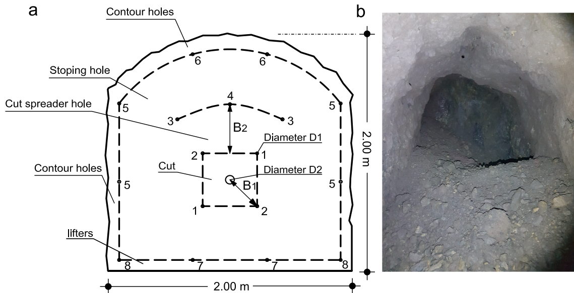
Fig. 2. Geometric drill pattern. (a) Blast pattern with 17 boreholes used in the tunnel of the present work based on the blasting manual, Geological and Mining Institute of Spain. (b) Front of a tunnel after a blast.
