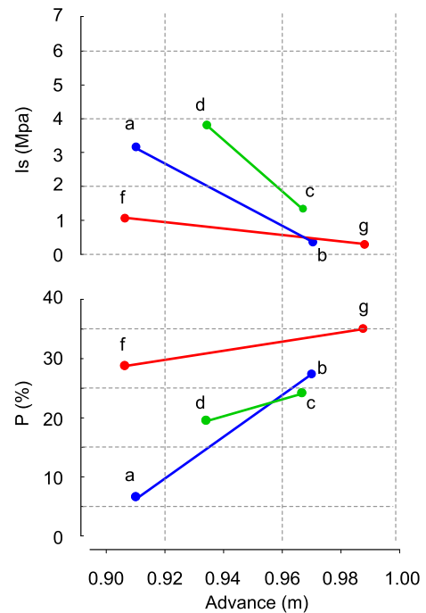
Fig. 5. Point load strength index I_s (MPa) and open porosity (%) versus advance (m). The lithotypes are: (a) aphanitic massive basalt, (b) altered and highly altered aphanitic massive basalt, (c) vacuolar aphanitic basalt, vacuole < 0.05 mm, (d) vacuolar aphanitic basalt, vacuole < 0.3 mm, (f) red colour ignimbrite and (g) highly altered red colour ignimbrite.
